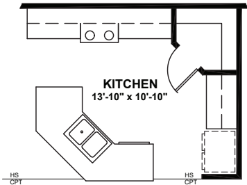
MAIN LEVEL OPTIONAL ALT KITCHEN ISLAND
