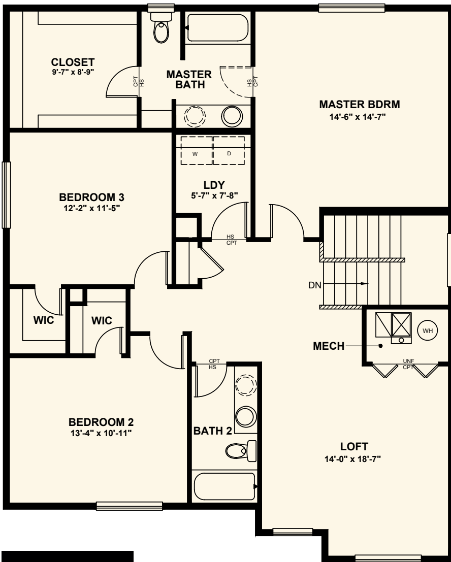
UPPER LEVEL OPTIONAL WALK-IN SHOWER W/ SEAT
