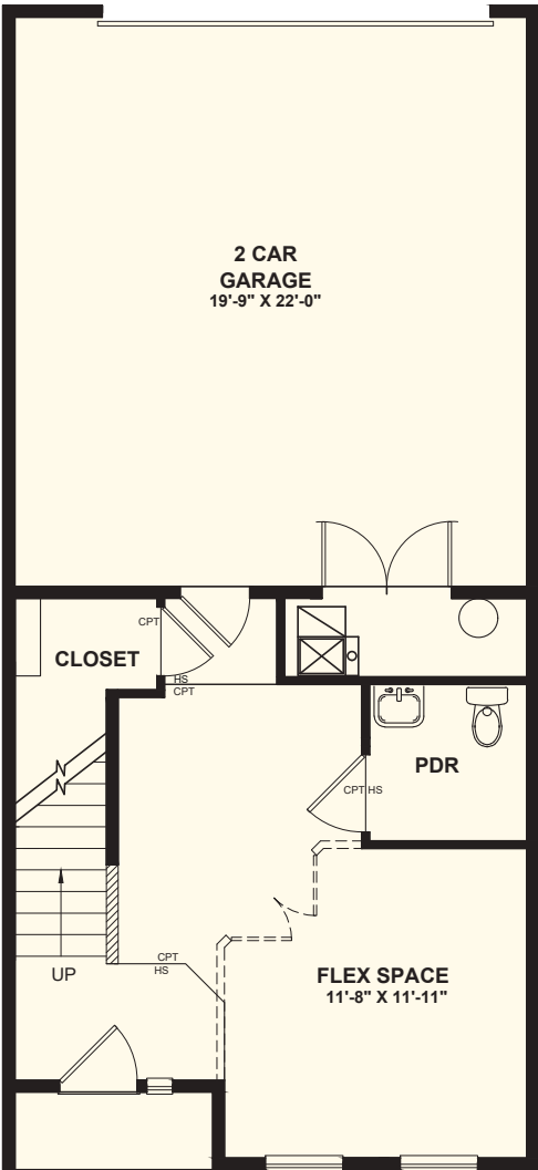
Lower Level 442 sf
