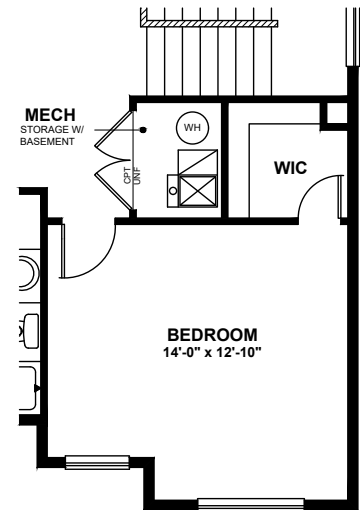
UPPER LEVEL OPTIONAL BEDROOM ILO LOFT
