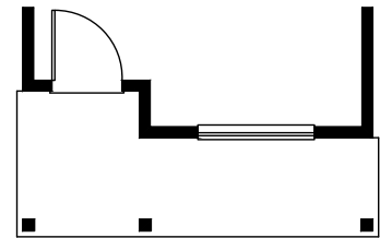
MAIN LEVEL OPTIONAL PORCH WITH "E" ELEV.
