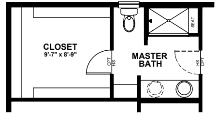
UPPER LEVEL OPTIONAL WALK-IN SHOWER W/ SEAT
