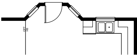
MAIN LEVEL OPTIONAL BAY WINDOW AT KITCHEN
