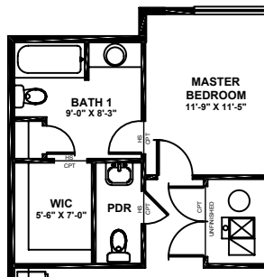
UPPER LEVEL - 1108 OPT. POWDER ROOM
