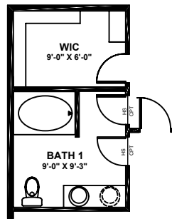
UPPER LEVEL - 1108 OPT. GARDEN TUB/SHOWER
