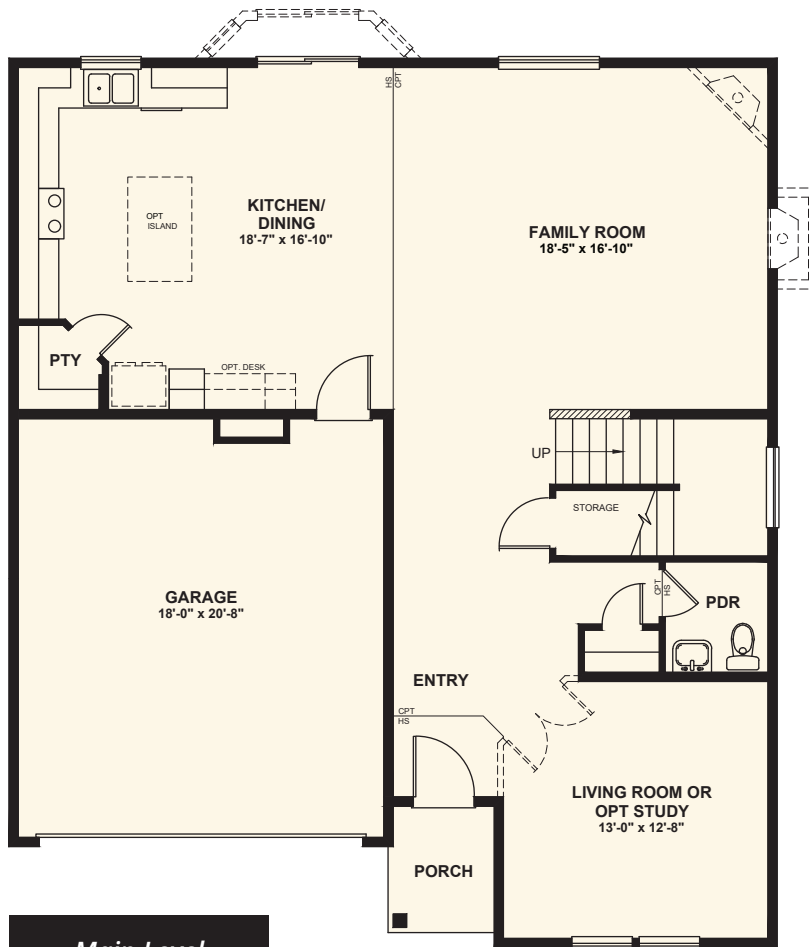
MAIN LEVEL OPTIONAL FRONT PORCH WITH ELEV. E
