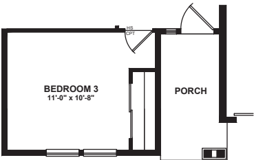
MAIN LEVEL OPTIONAL FRONT PORCH WITH MODERN PRAIRIE ELEV.
