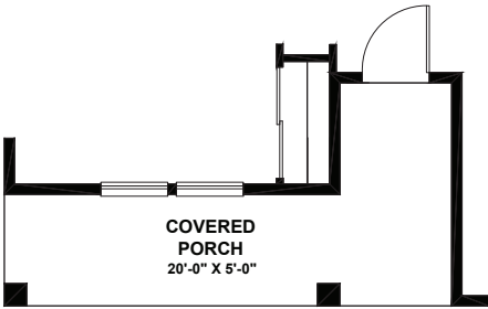
MAIN LEVEL PORCH WITH OPTIONAL ELEVATIONS "B" & "C"
